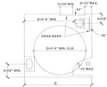
PLAN VIEW - TOILET ROOM
