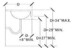
DETAIL - LAVATORY
